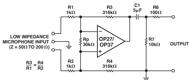
Figure 9. Fixed Gain Transformerless Microphone Preamplifier
